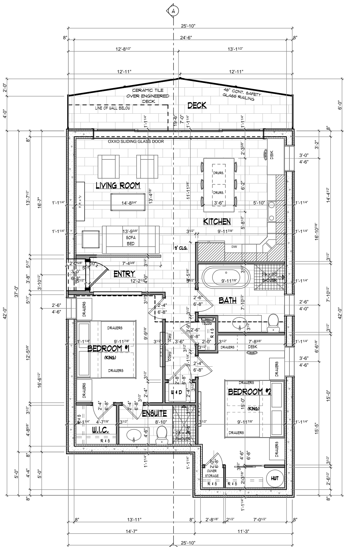
29B MIDDLE LEVEL PLAN
